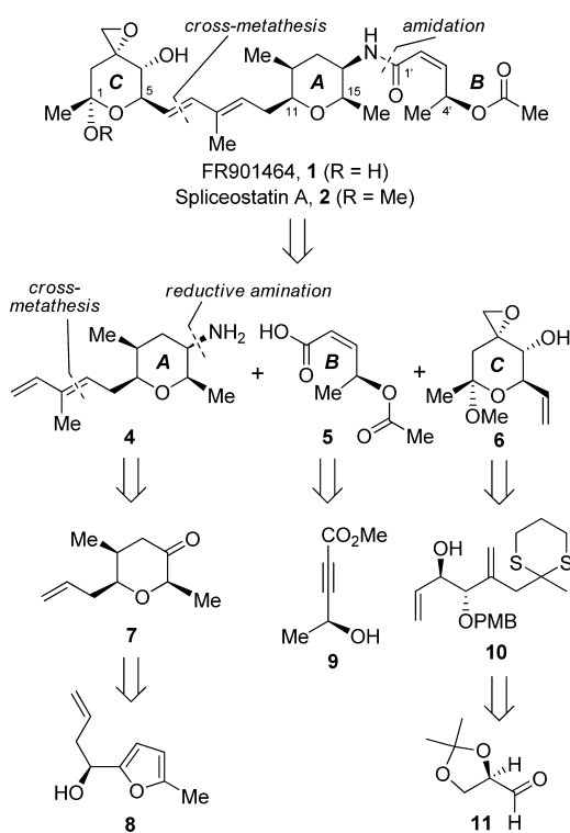
Scheme 1. Retrosynthetic Analysis of FR901464 and Spliceostatin A
